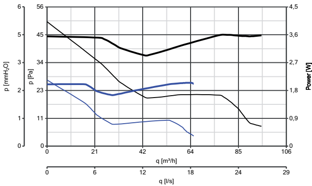
ME 100/4" cod. 11268
